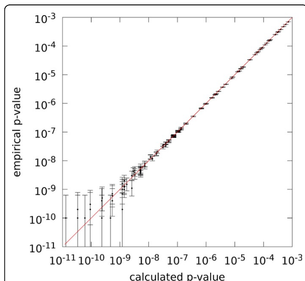
Figure 1 Comparison of empirical and calculated p-values for bacterial genomes. Comparison of empirical and calculated p-values for gene clusters from four bacterial genomes (log-log plot, N = 182 ). Pearson correlation of log-log-pairs is r = +0.9976775 ( r^2 = 0.9953604 ), coefficient of determination of log-log-pairs is R^2 = 0.9951661 (identity in red). Error bars visualize the 95% Agresti-Coull confidence interval.
