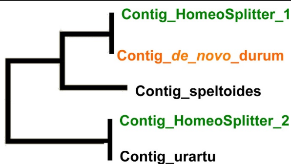
Figure 4 Phylogenetic tree inferred on homologous contigs from cluster 6960. The original contig obtained by de novo assembling (contig_ de_novo_durum ) was more similar to the speltoides contig (contig_ speltoides ) than to the urartu one (contig_ urartu ). After using HomeoSplitter we obtained the most expressed split contig (contig_HomeoSplitter_1) that is still similar to the speltoides one and one less expressed contig (contig_HomeoSplitter_2) highly similar to the urartu one.
